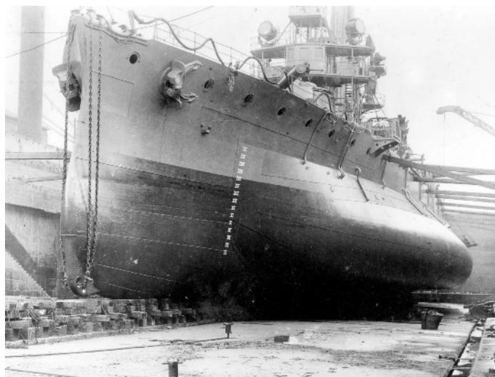
HMS Glatton undergoing conversion. Note the extent of the anti-torpedo bulges ( www.destinationsjourney.com )
